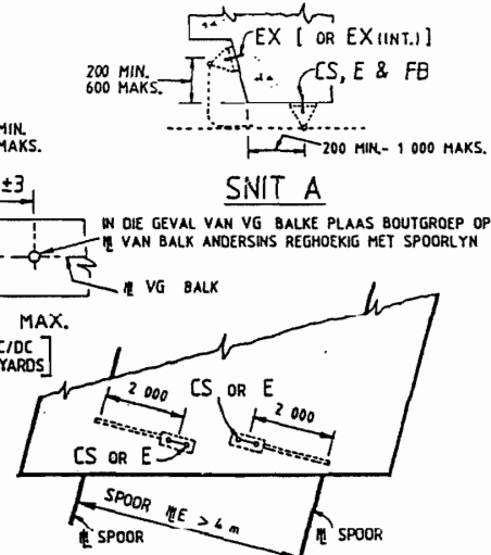
PLAN 'B' (TRACK CRS. > 4 m) (FURTHER DETAILS AS FOR PLAN 'A')
