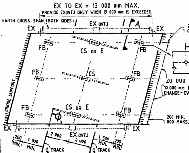
PLAN 'A' (TRACK CRS. = 4 m)
