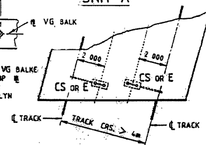
PLAN 'B' (TRACK CRS. > 4m) (FURTHER DETAILS AS FOR PLAN 'A')
